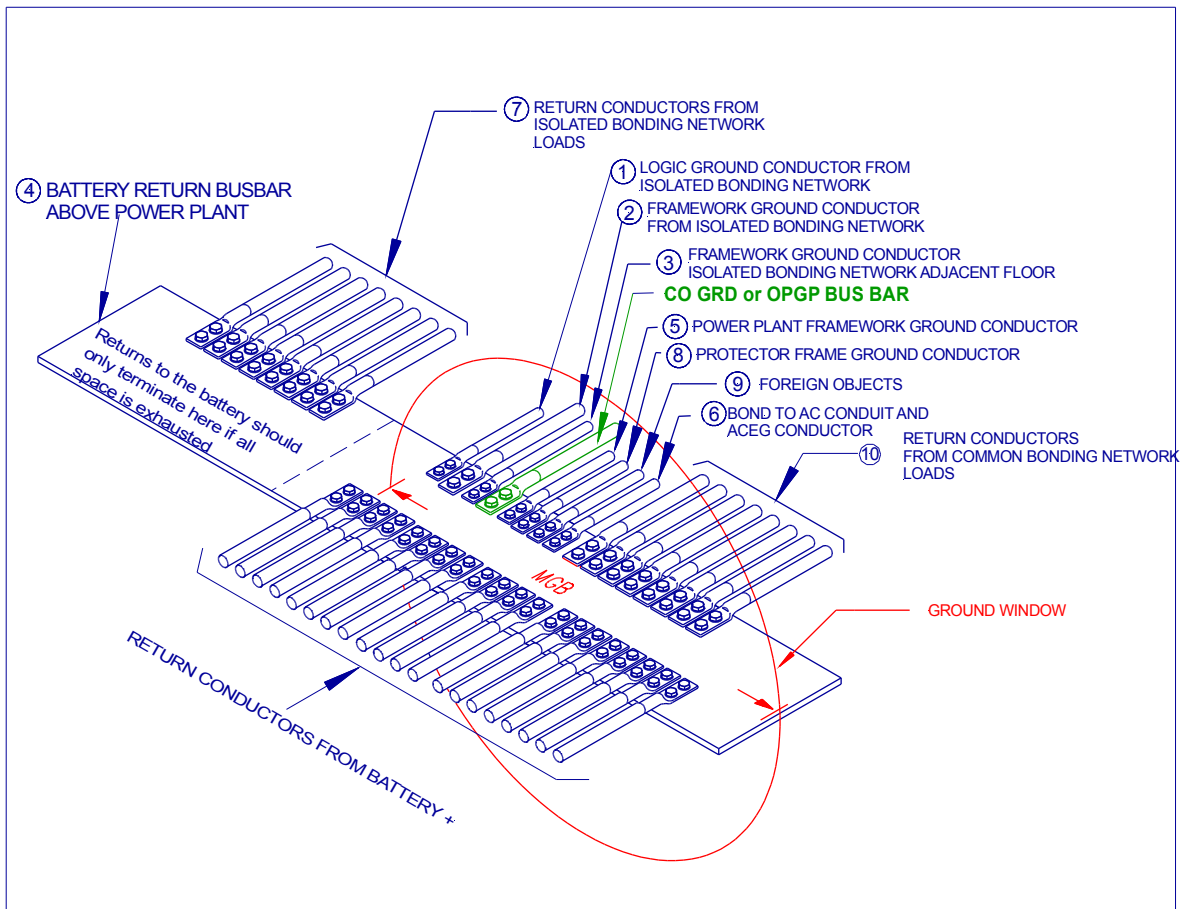
Figure 4-5 Sequencing of Conductors Along an MGB that is Part of a Power Plant's Battery Return Bus
