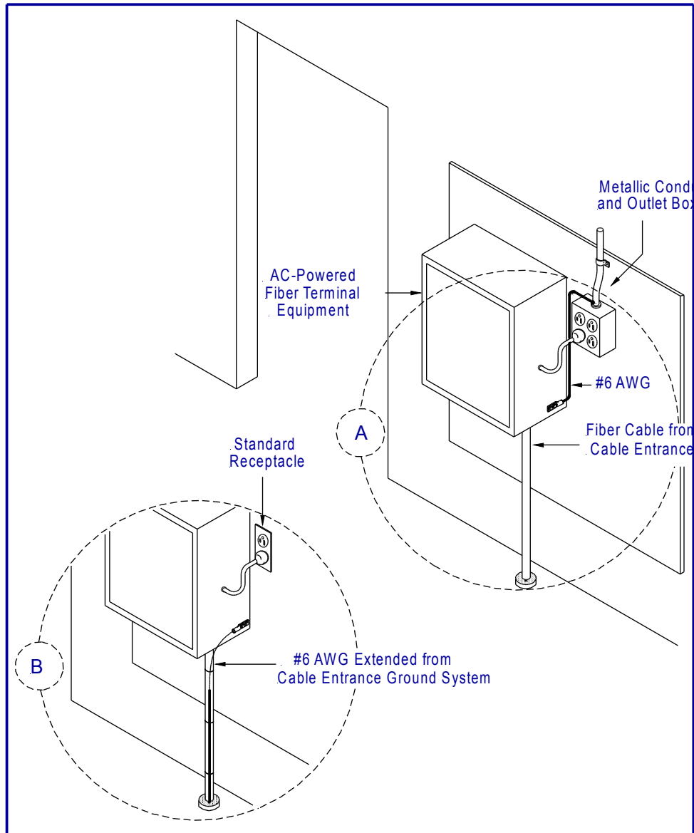
Figure 5-5 Grounding Arrangements for Wall-Mounted Customer Premises Equipment
