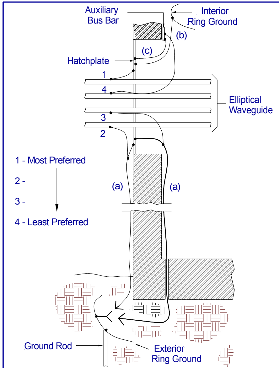
Figure 6-7 Preferred Bonding Locations
