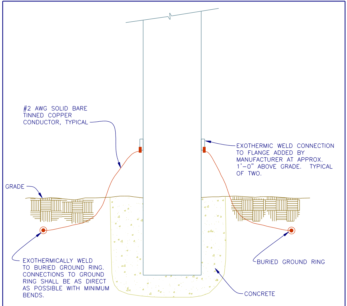
Figure 7-5 Buried Monopole Grounding Detail
