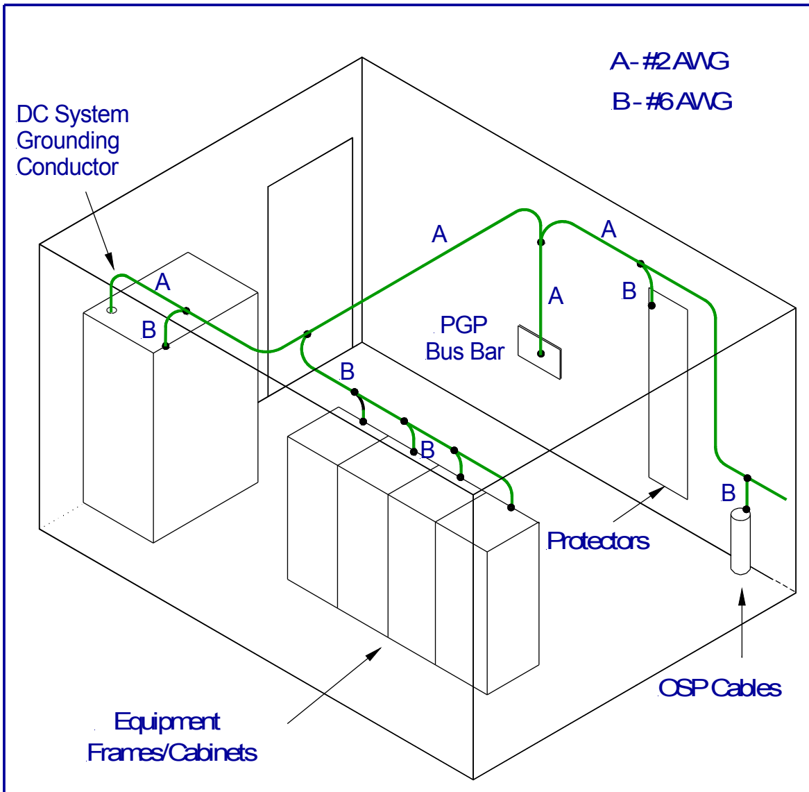
Figure 5-3 Typical Grounding Conductor Arrangement in an EEE (hut shown)
