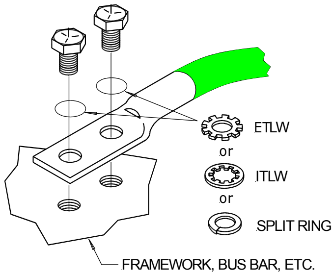
Figure 1-4 Application of Lockwashers
