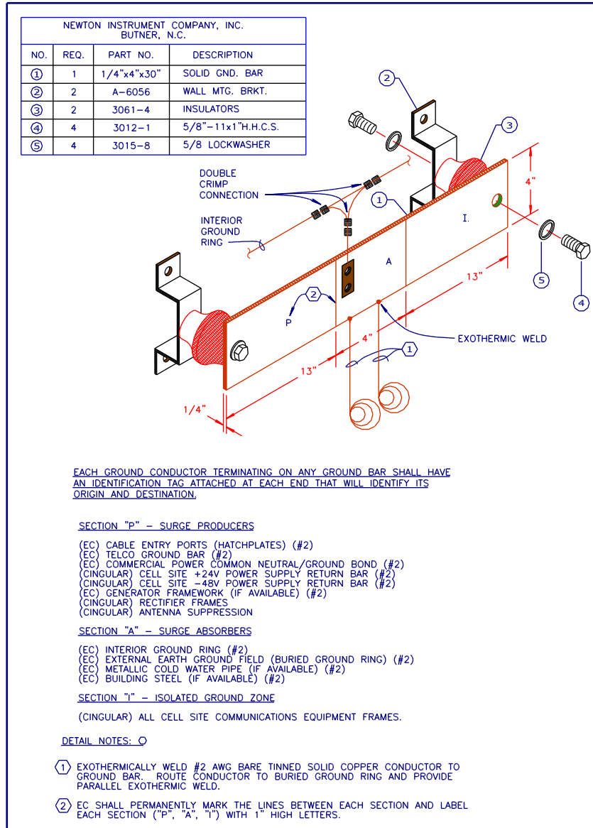
Figure 7-11 Cell Reference Ground Bar (Stand Alone Cell Site) - CRGB Detail
