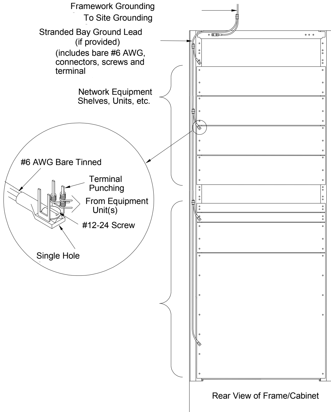
Figure 3-3 Network Equipment Frame/Cabinet Grounding Details
