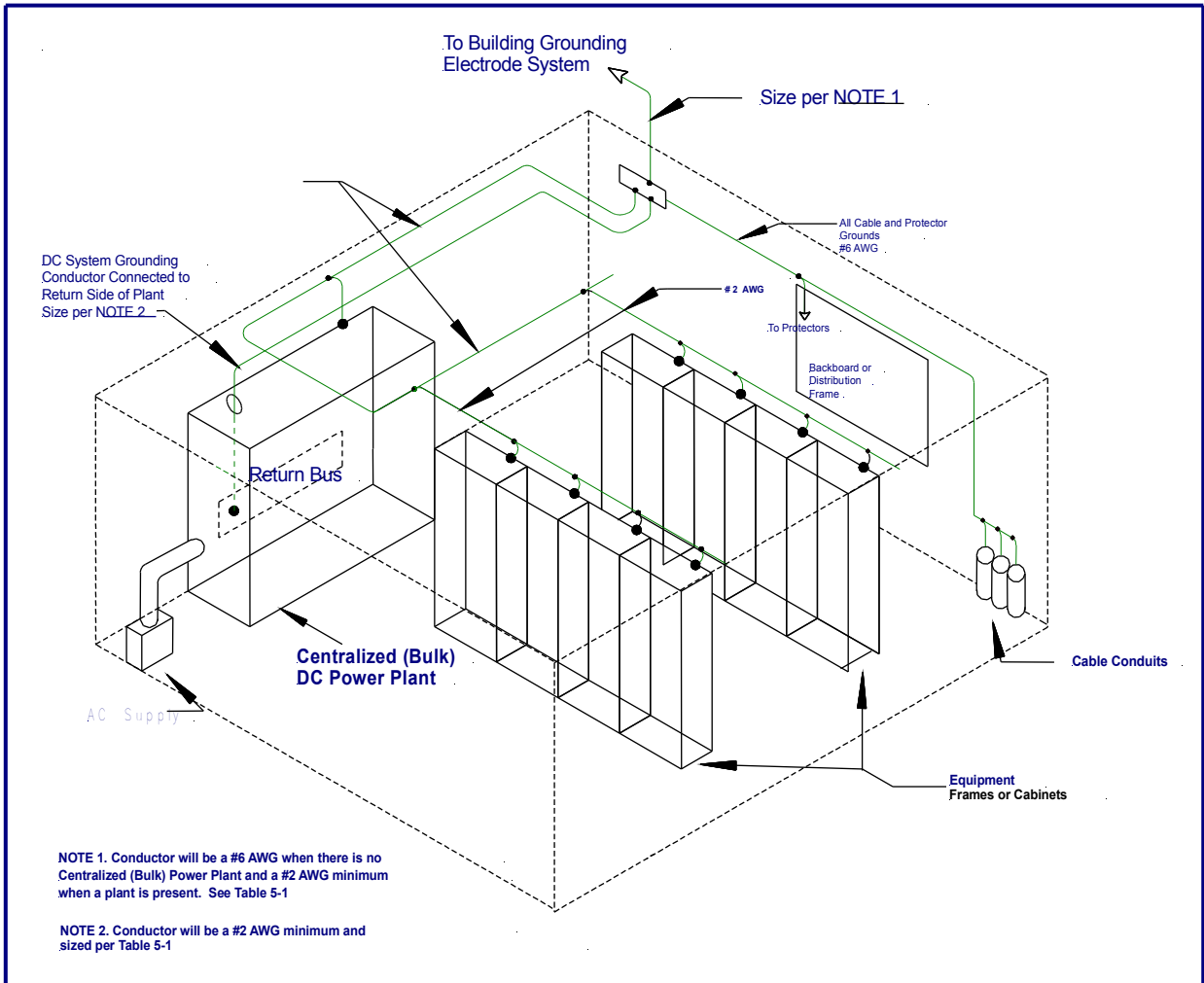
Figure 5-4 Typical Grounding Arrangement for Customer Premises Telephone Room
