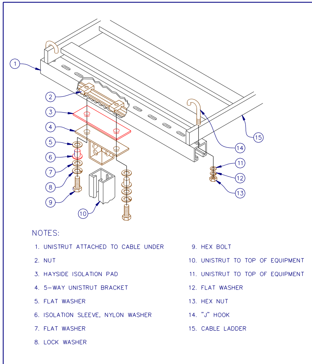
Figure 7-14 Cable Tray Insulation Detail
