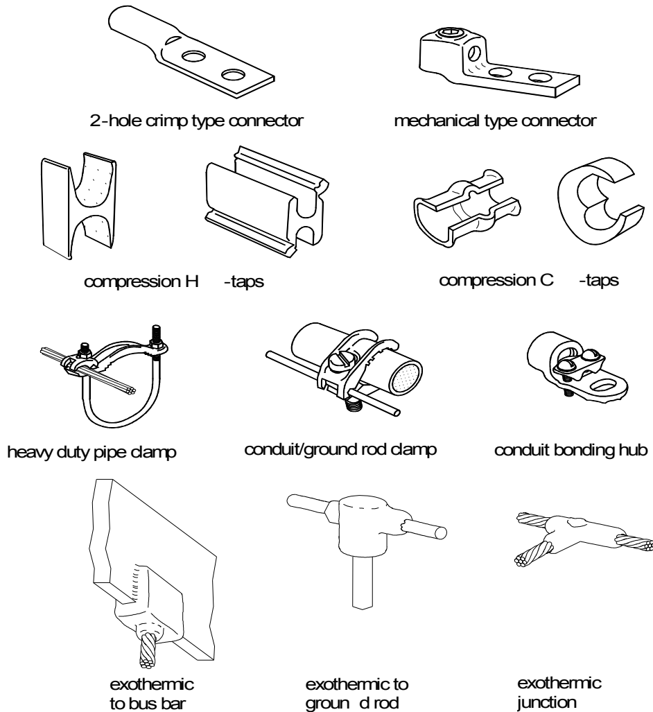
Figure 1-2 Typical Conductor Terminations
