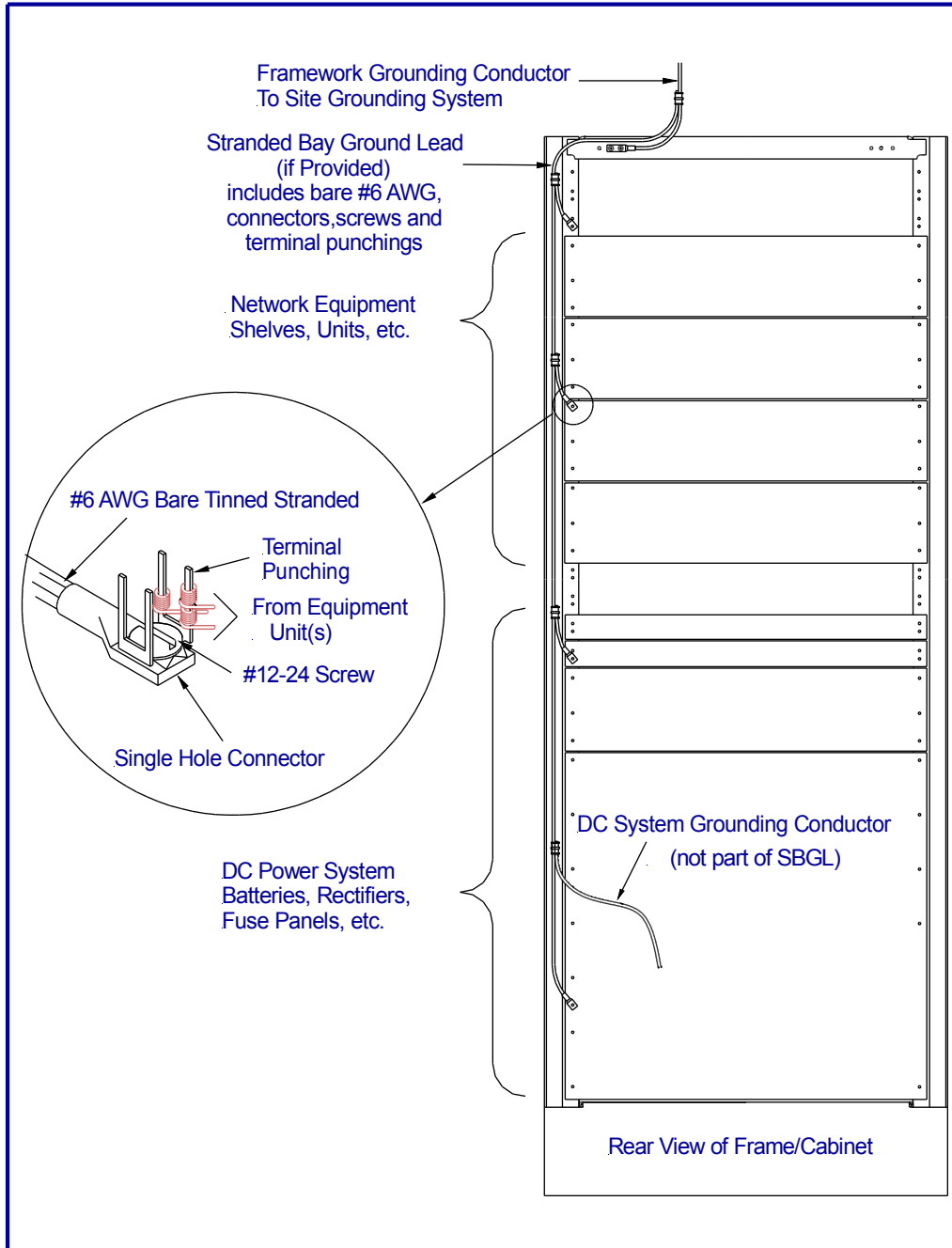
Figure 5-6 Network Equipment Frame/Cabinet Grounding Details
