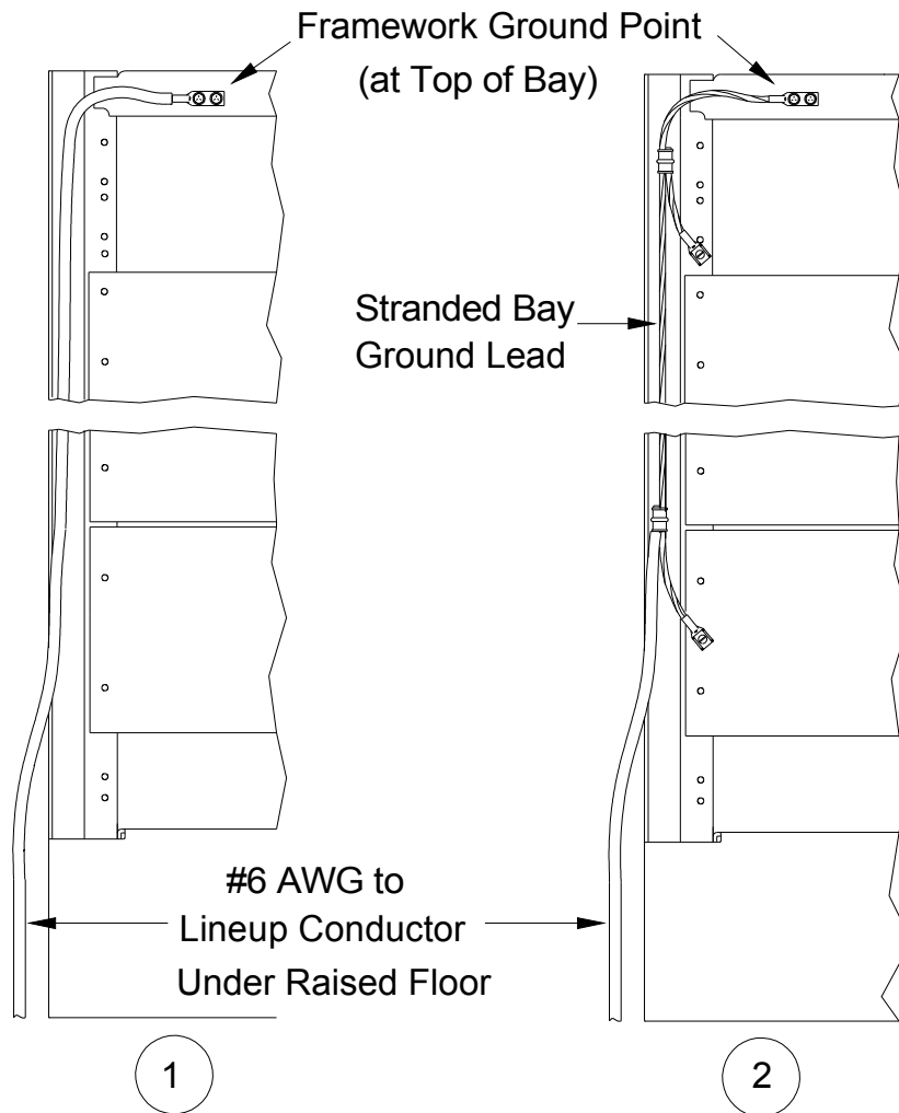
Figure 3-5 Methods of Connecting Between Lineup and Framework Ground
