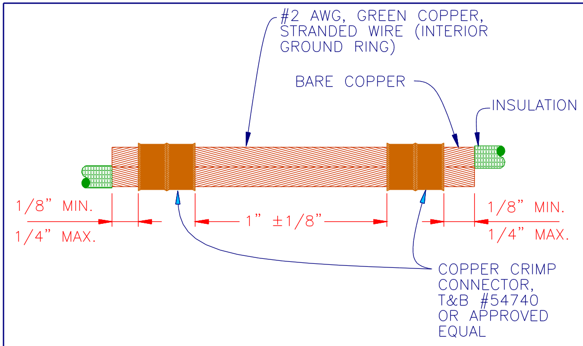
Figure 7-8 Ground Ring Splice Detail
