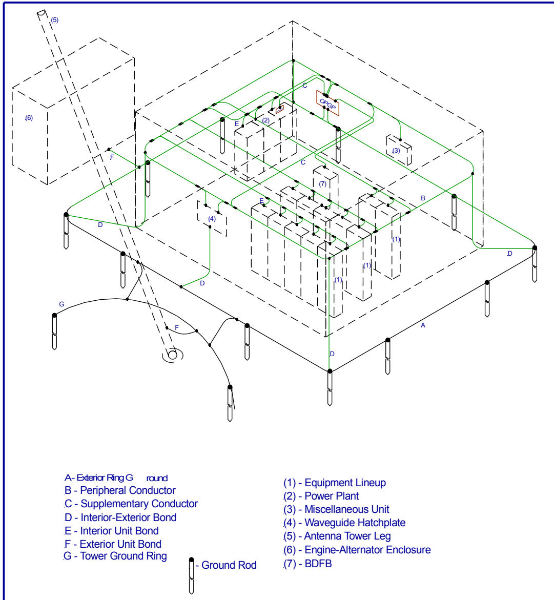
Figure 6-1 Typical Radio Site Grounding System
