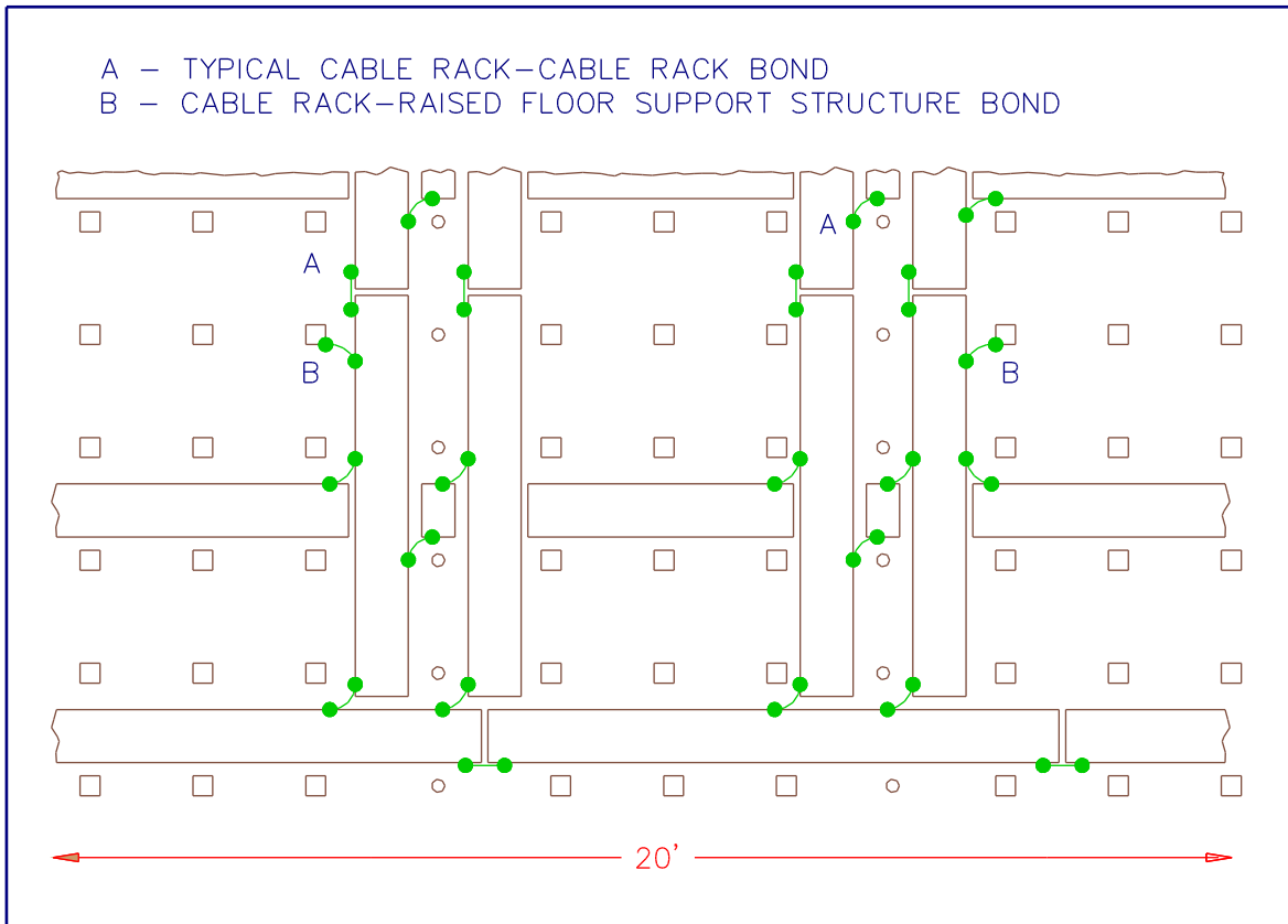
Figure 3-6 Typical Bonding Required When Cable Rack is not Secured to the Raised Floor Support Structure
