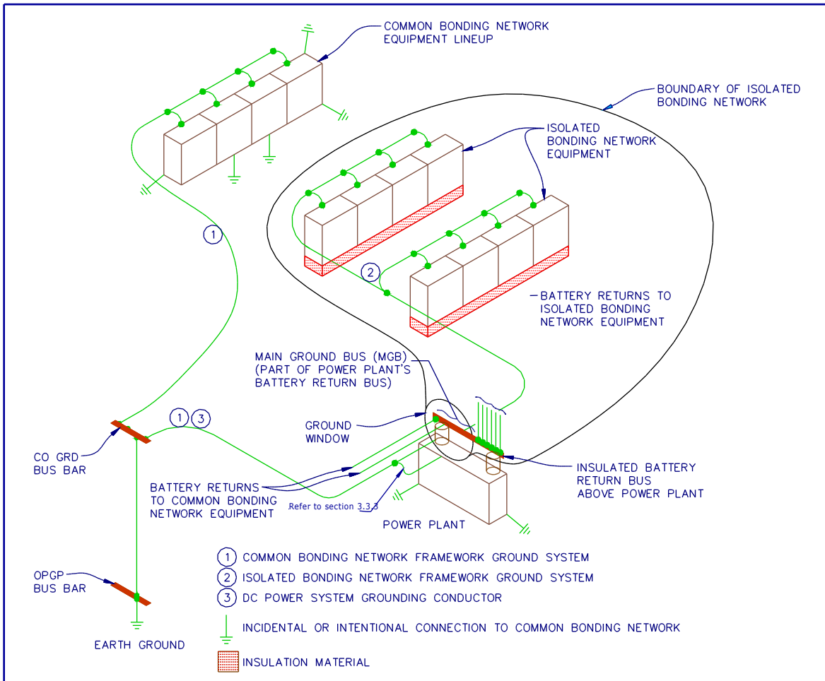
Figure 4-2 Relationship Between Common and Isolated Bonding Networks (MGB is located at power plant)
