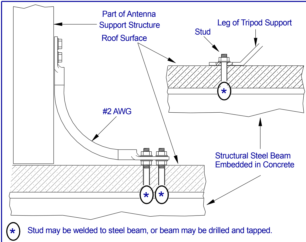
Figure 6-8 Bonds to Structural Steel
