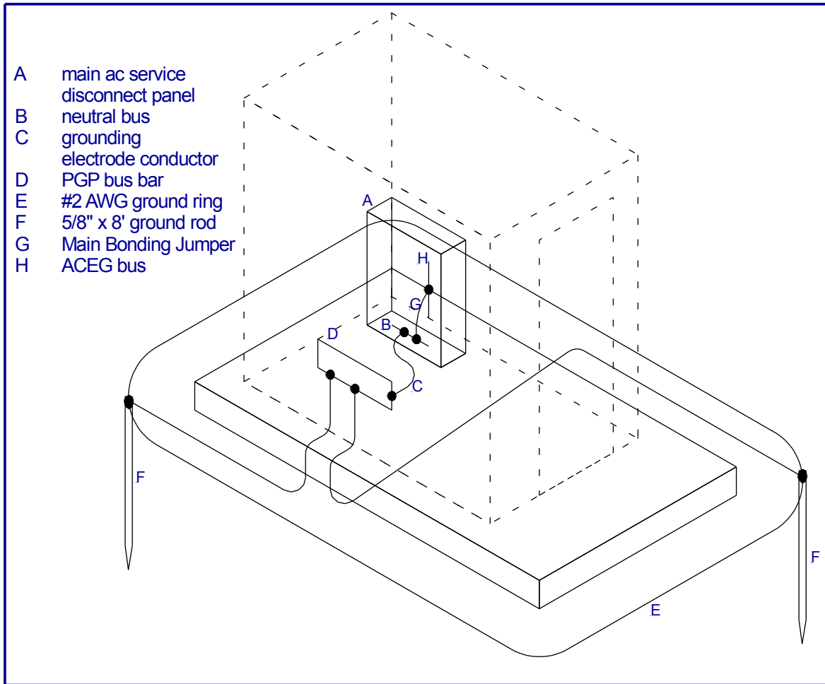
Figure 5-1 Earth Electrode System and AC Service Grounding (hut shown)
