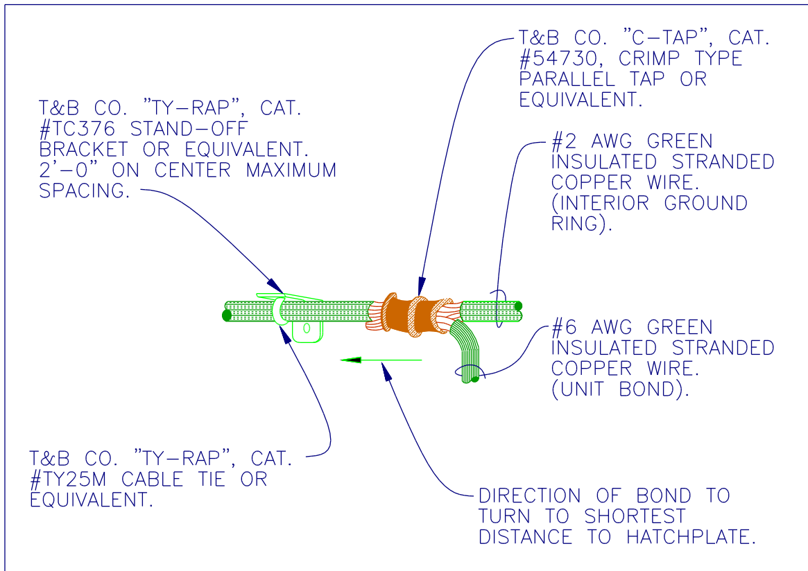
Figure 7-9 Interior Ground Ring Wall Support Detail
