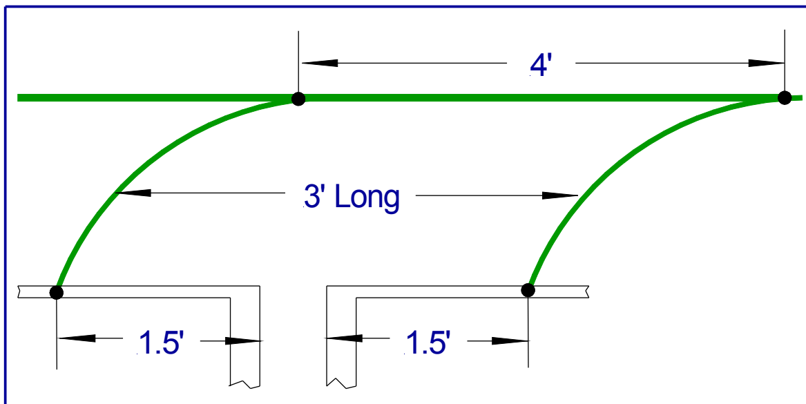
Figure 6-5 Determining the Distance Between Metallic Objects
