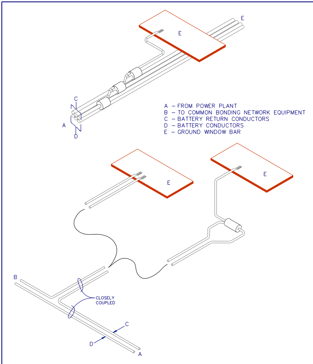
Figure 4-10 Methods of Bonding Battery Return Conductors to the MGB
