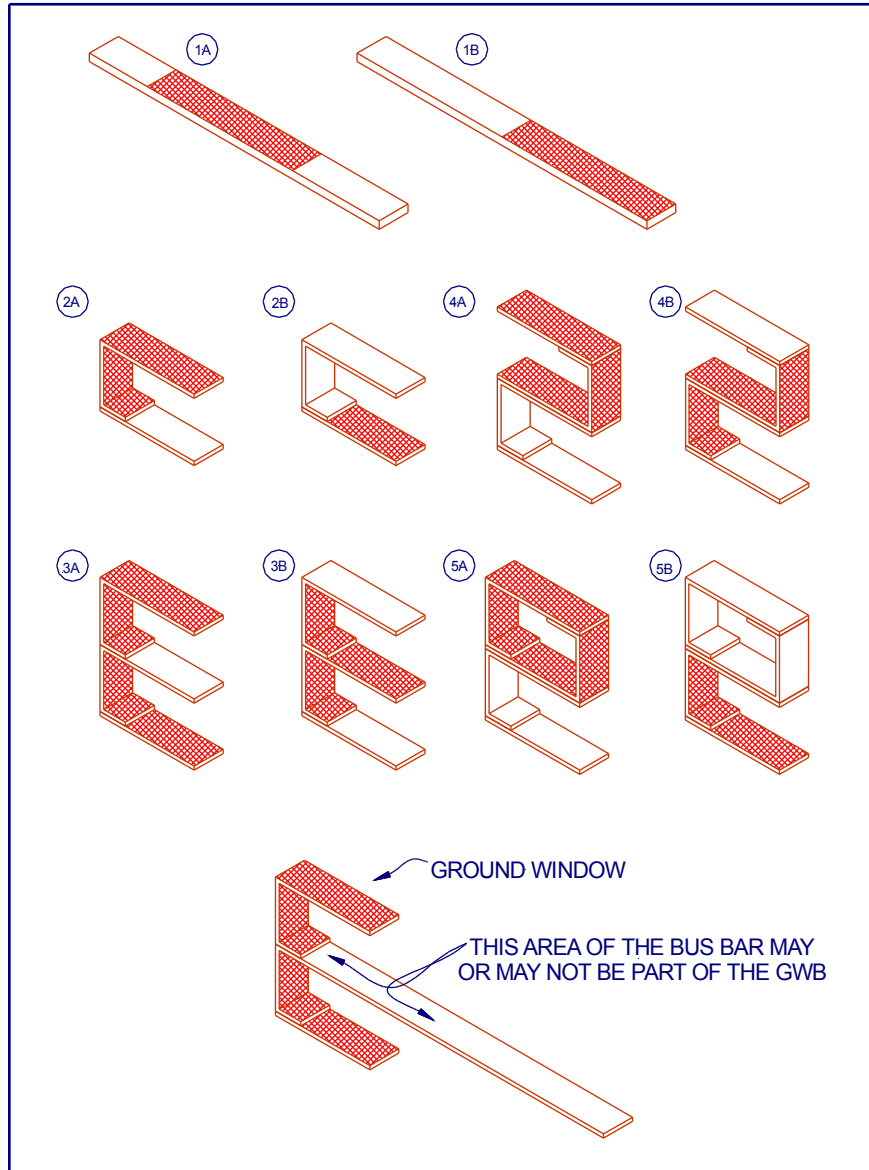
Figure 4-4 Examples of Battery Return Bus Bar/MGB Arrangements
