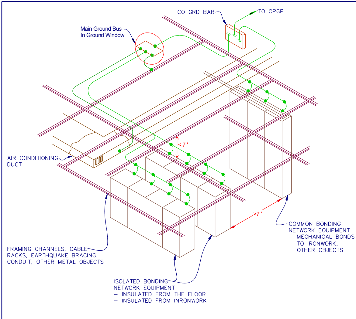
Figure 4-7 Foreign Object Bonds to Nearby Metallic Objects
