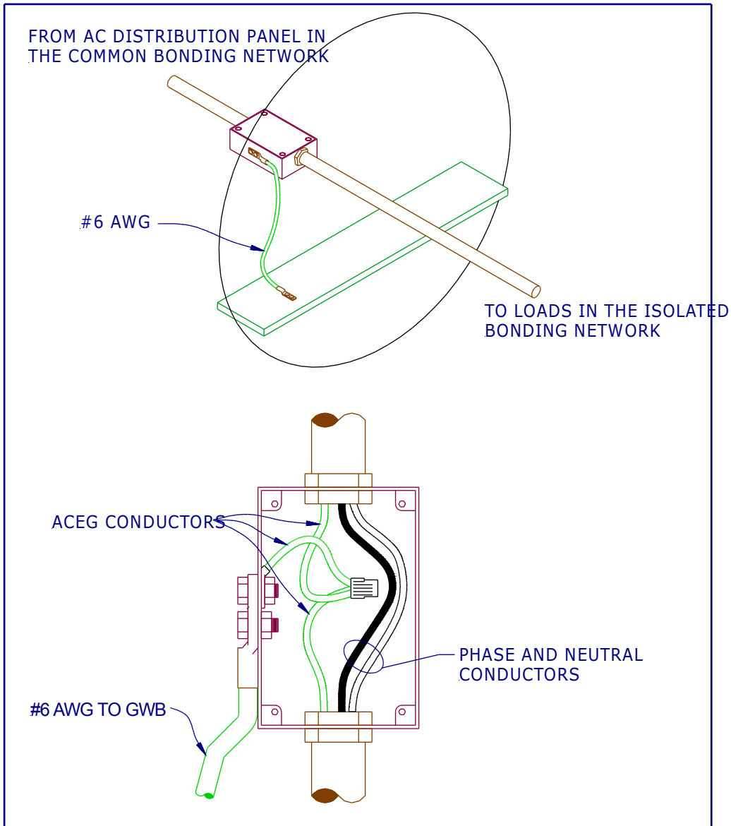
Figure 4-6 Bonding of Conduit and ACEG Conductors to MGB
