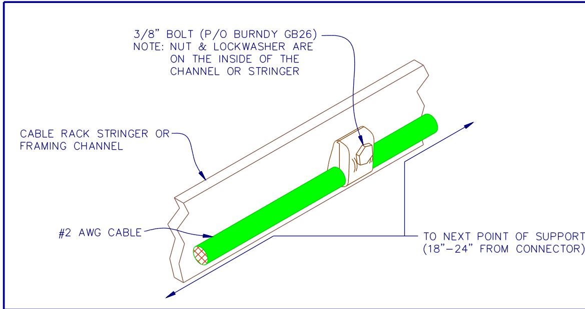
Figure 6-3 Method of Bonding Supplementary Conductor to a Framing Channel
