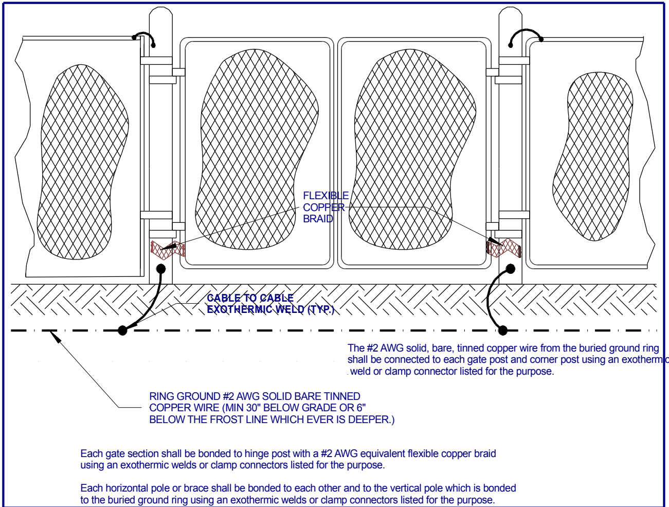
Figure 6-4 Fence and Gate Grounding for Antenna Towers
