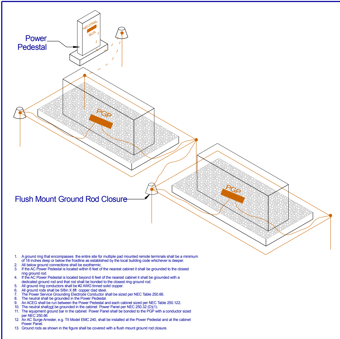
Figure 5-2(a) Two Individual Pad mounted cabinets installed separately utilizing the same Power Pedestal
