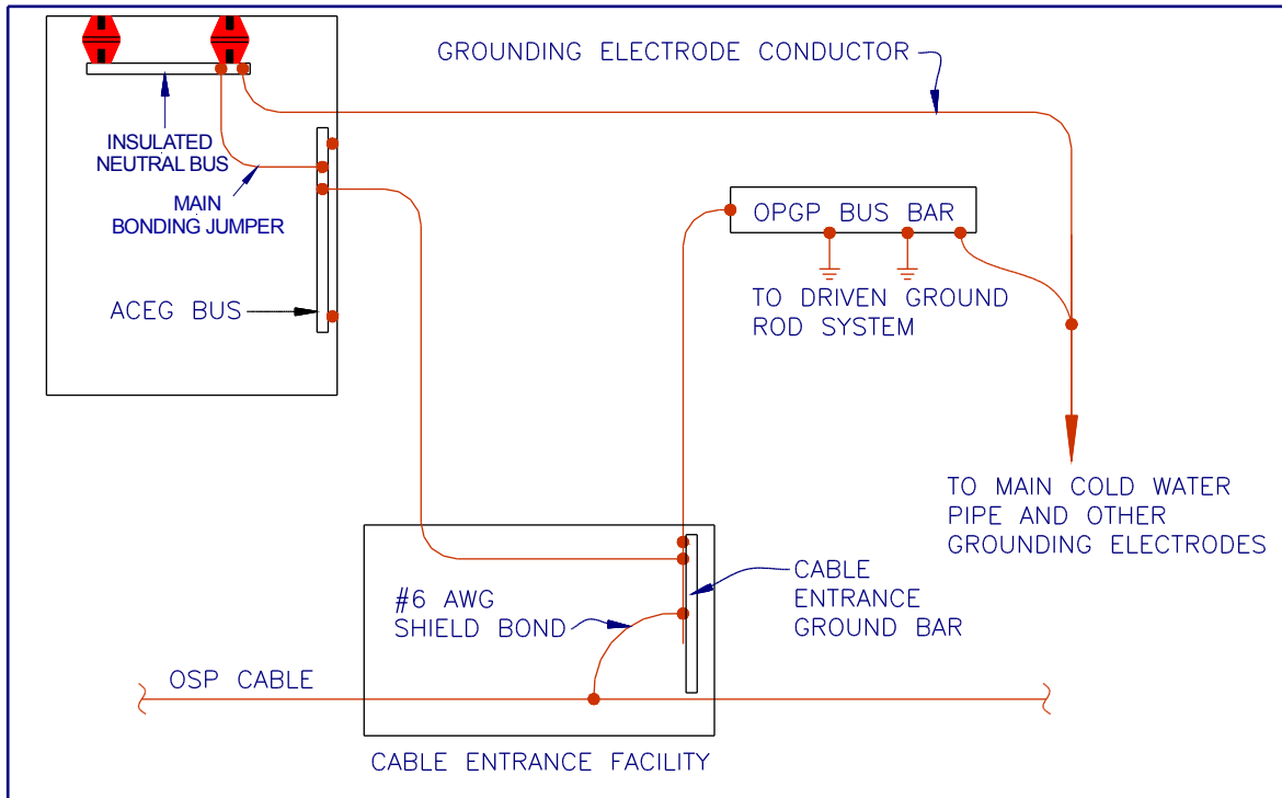
Figure 2-4 Typical Interbonding Arrangement
