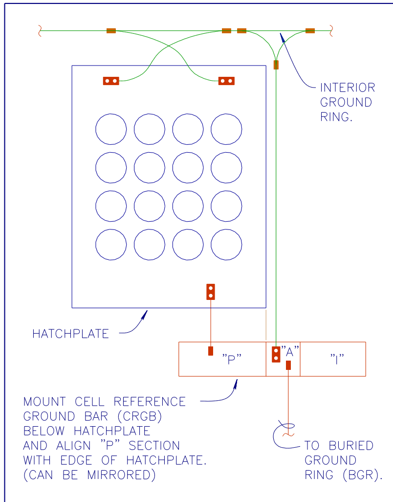
Figure 7-13 Cell Reference Ground Bar (CRGB) Installation Detail
