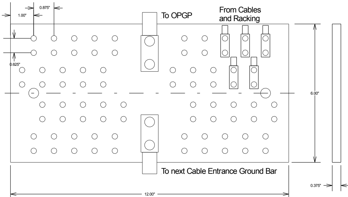
Figure 3-4 Typical Cable Entrance Ground Bar
