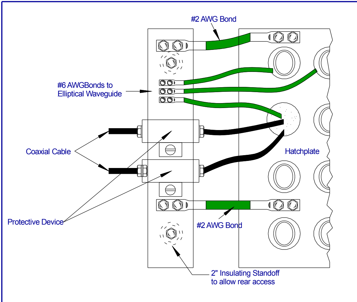
Figure 6-6 Auxiliary Bus Bar Details
