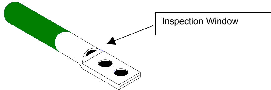
Figure 1-1 Compression Connector with Inspection Window
