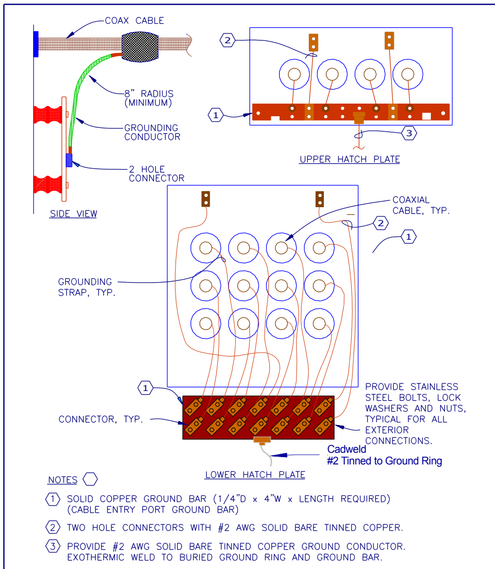
Figure 7-17 Exterior Hatch-plate Grounding (Cable Entry Port) Detail
