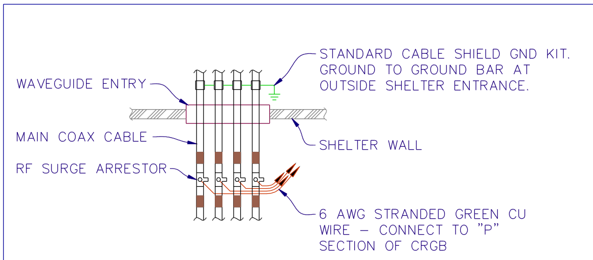
Figure 7-17a RF Surge Arrester Detail
