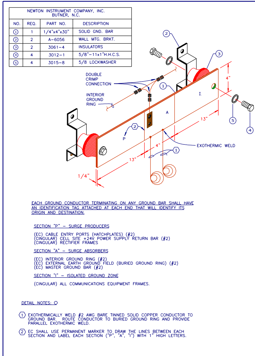
Figure 7-12 Cell Reference Ground Bar - CRGB Detail Co-Located at MSC
