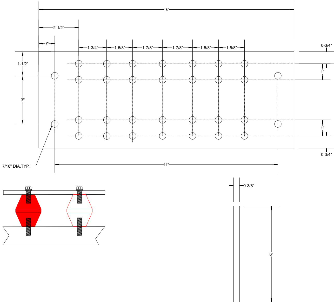
Figure 1-3 Typical Central Office Ground Bar
