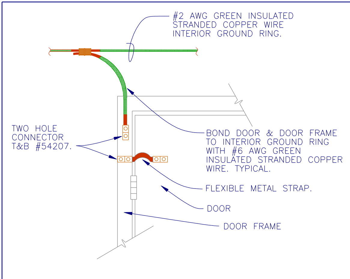
Figure 7-10 Door Grounding Detail
