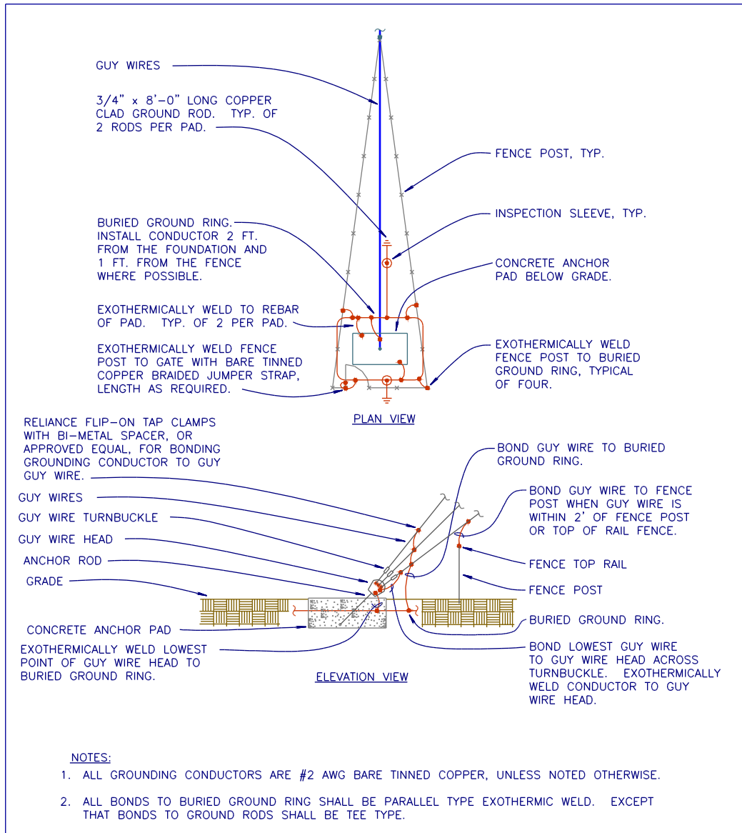
Figure 7-6 Guy Wire Grounding Detail
