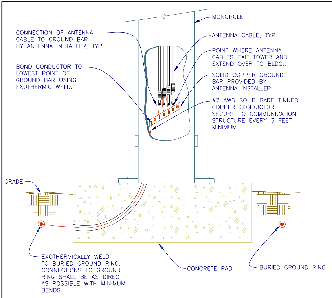
Figure 7-15 Monopole Cable Grounding Detail
