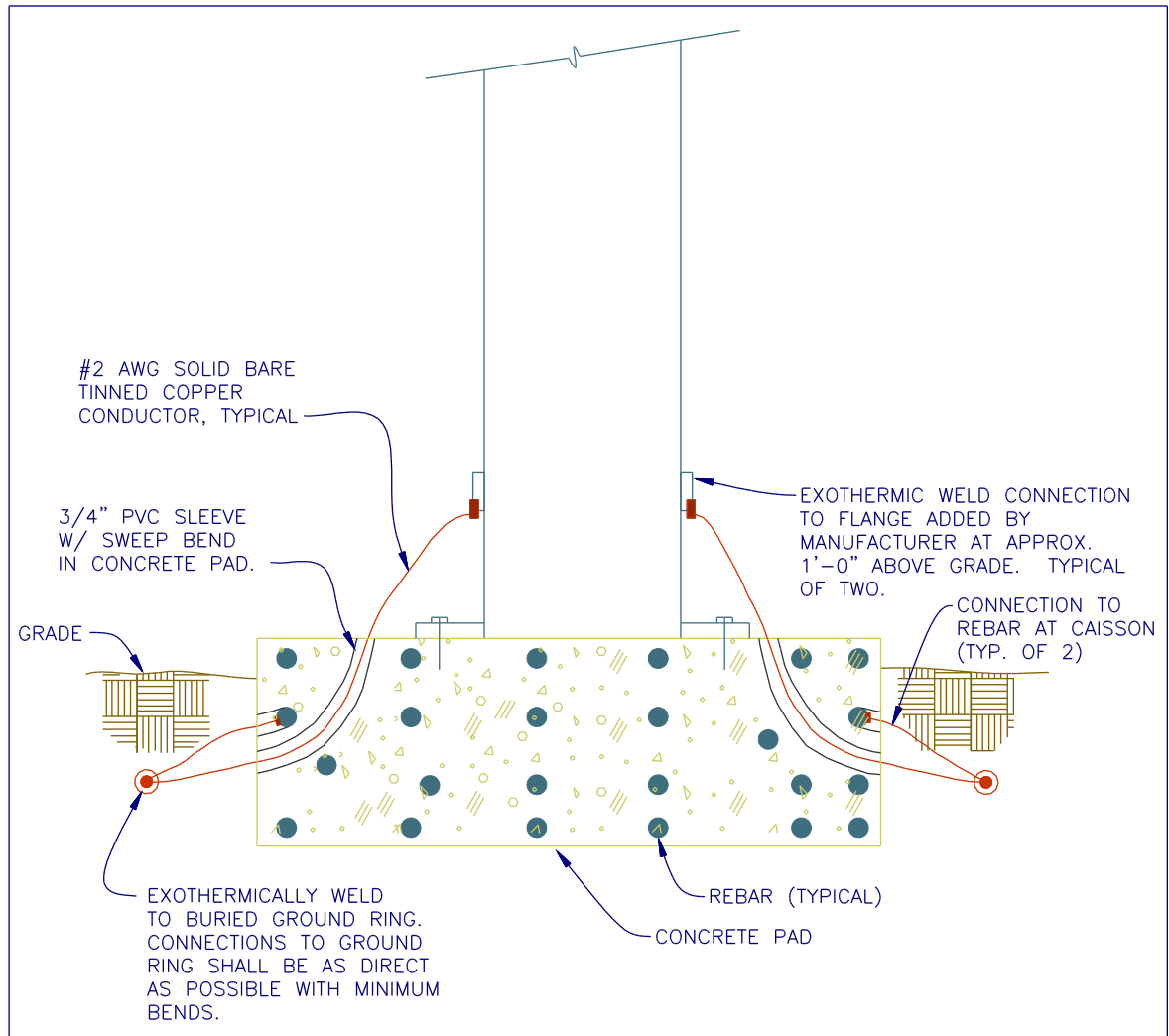
Figure 7-4 Monopole Grounding Detail
