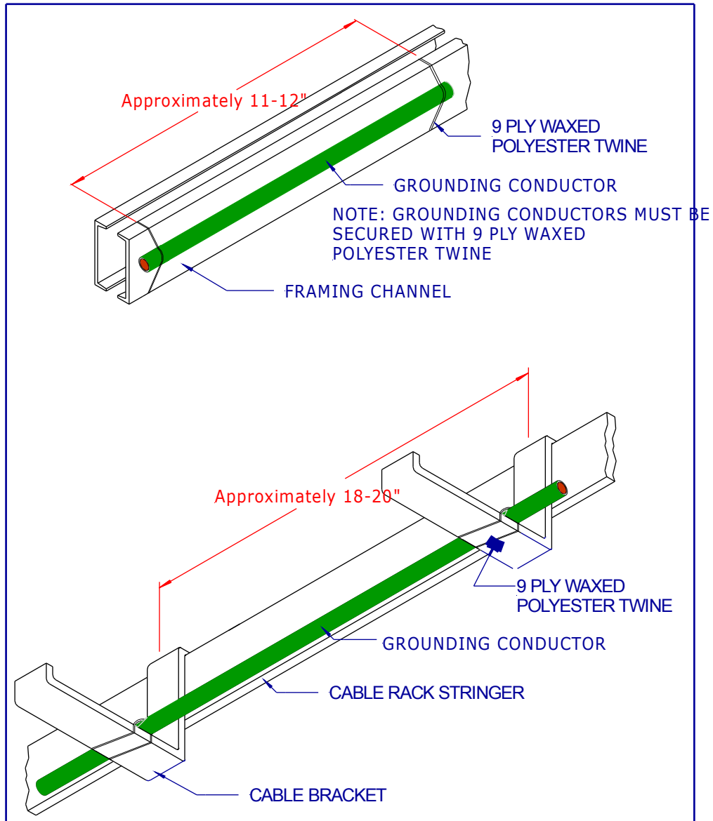
Figure 1-4 Use of Lacing to Secure Grounding Conductors
