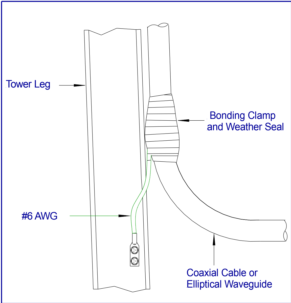
Figure 6-2 Bond to Tower Leg
