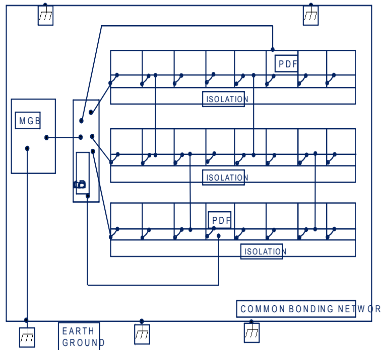
Figure 4-9(b) Lucent 5ESS IBN with 5EFGB
