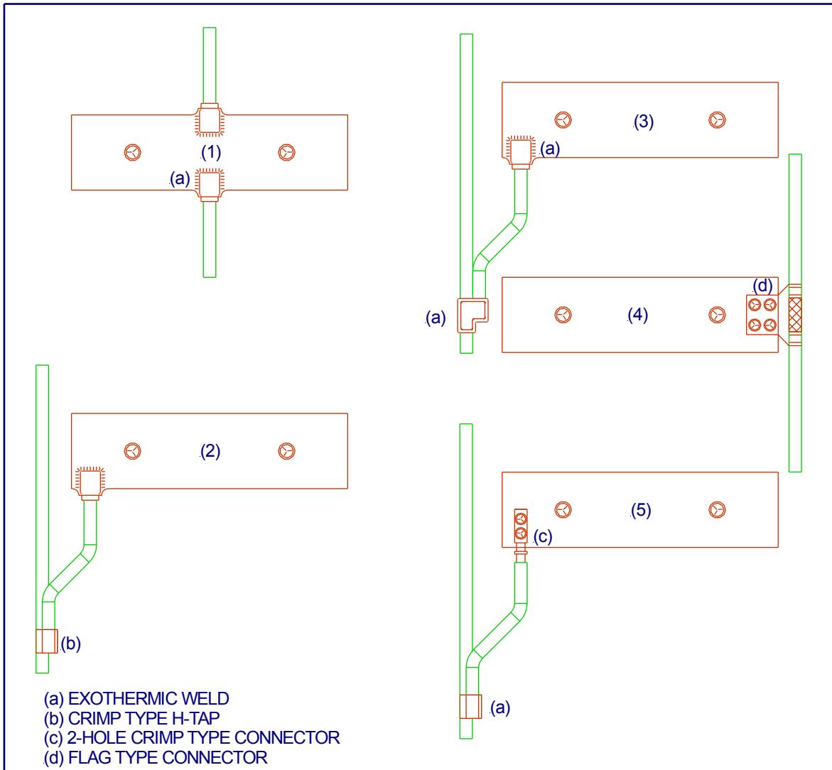
Figure 2-7 Methods of Connecting 750 kcmil Vertical Riser to CO GRD Bus Bar
